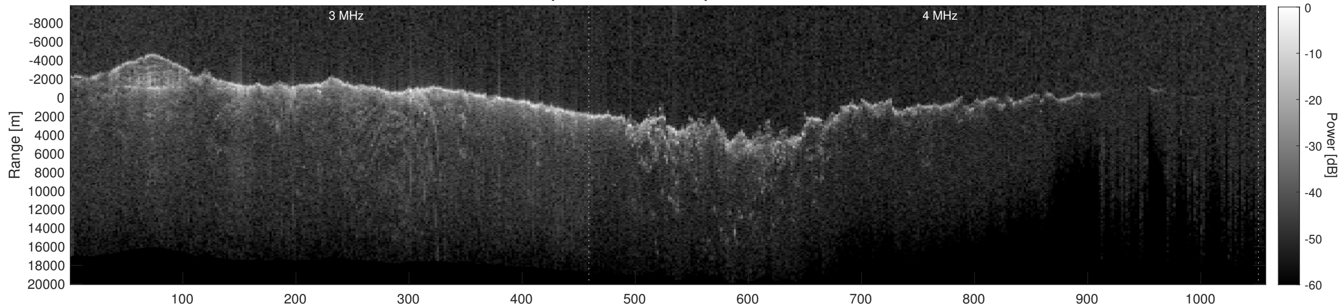
Orbit 10559, Depth-Corrected Cluttergram
