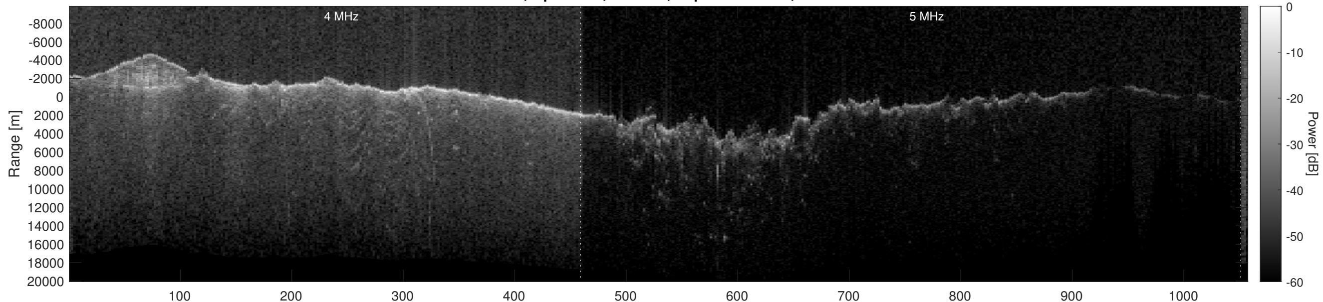
Orbit 10559, Optimized, Window, Depth-Corrected, Channel 2
