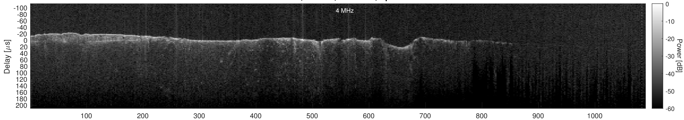
Orbit 10561, Cluttergram
