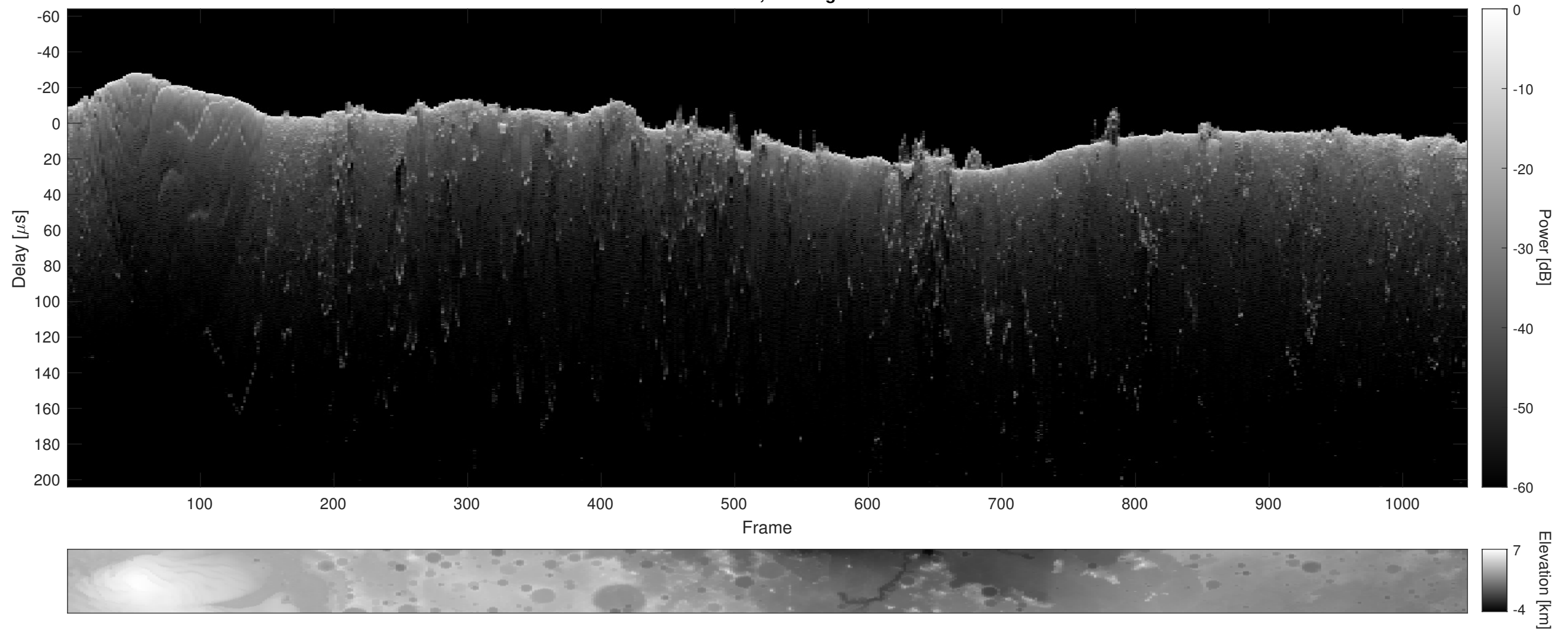
Orbit 10562, Cluttergram
