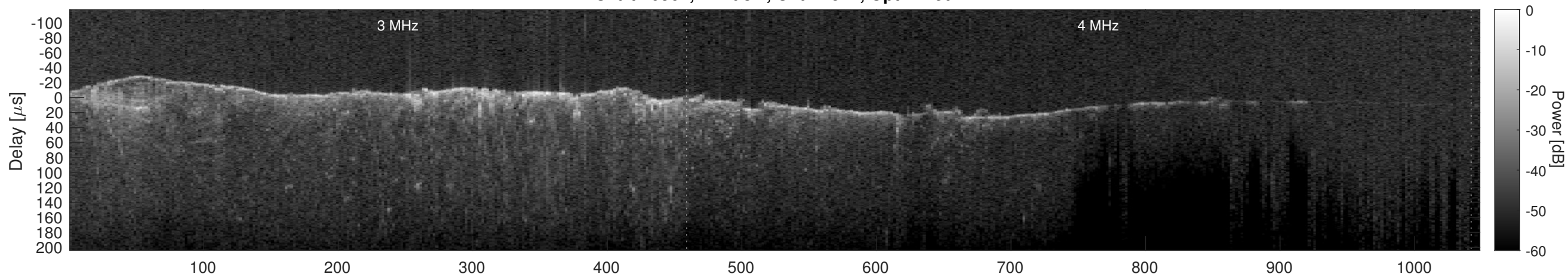
Orbit 10562, Cluttergram
