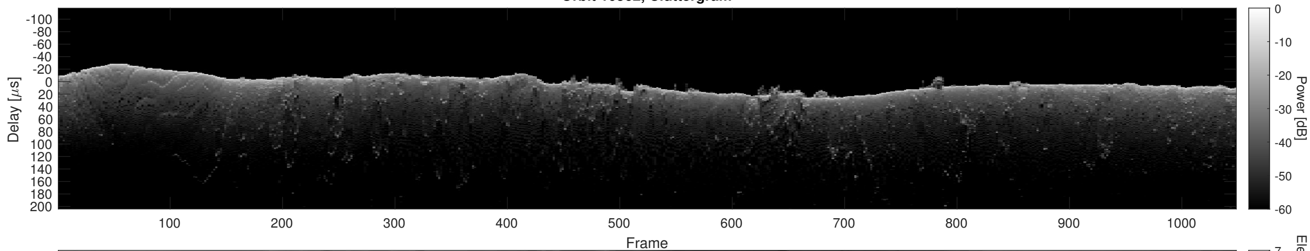
Orbit 10562, Cluttergram
