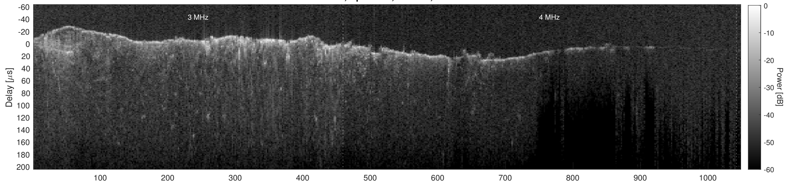
Orbit 10562, Cluttergram
