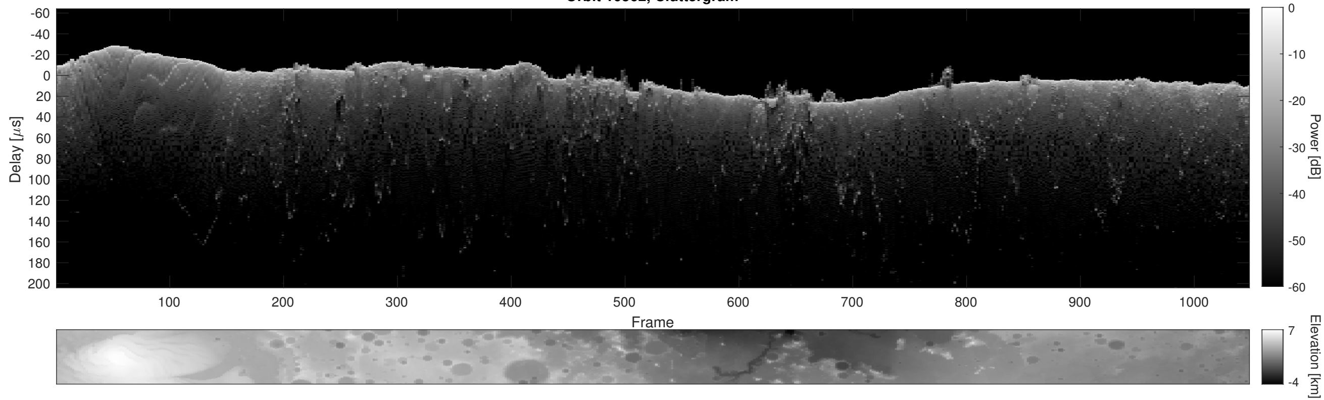
Orbit 10562, Cluttergram
