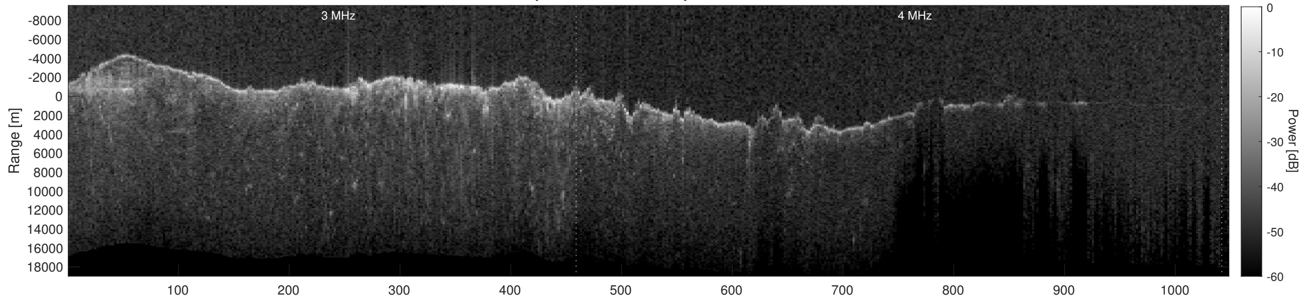
Orbit 10562, Depth-Corrected Cluttergram
