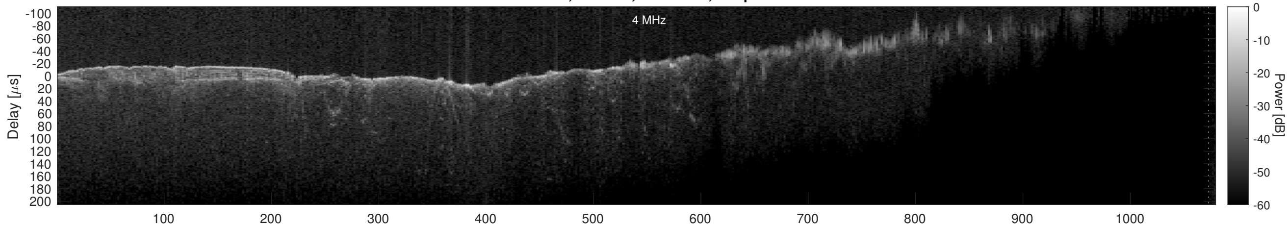
Orbit 10568, Window, Channel 2, Optimized
