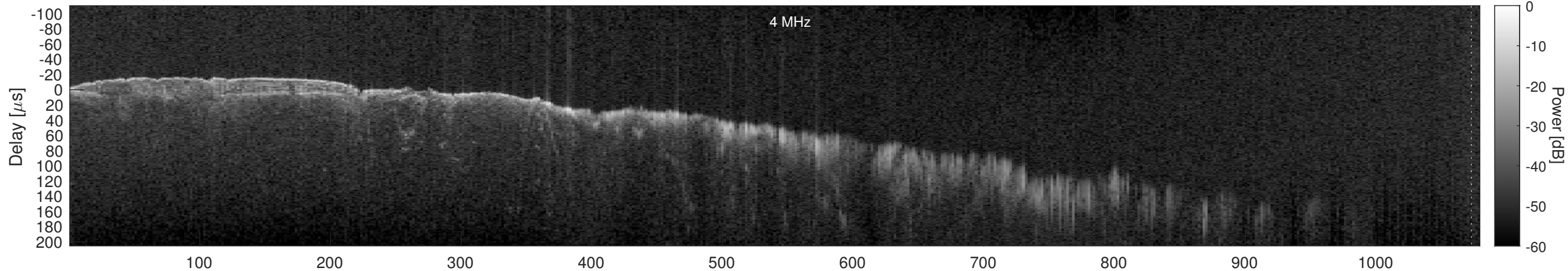
Orbit 10568, Window, Channel 2, Chapman
