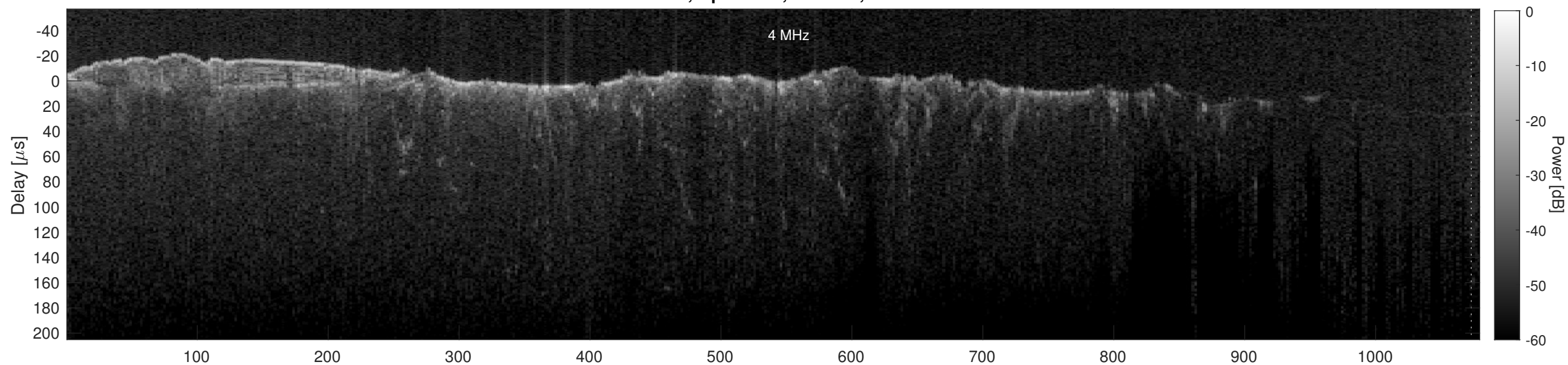
Orbit 10568, Cluttergram
