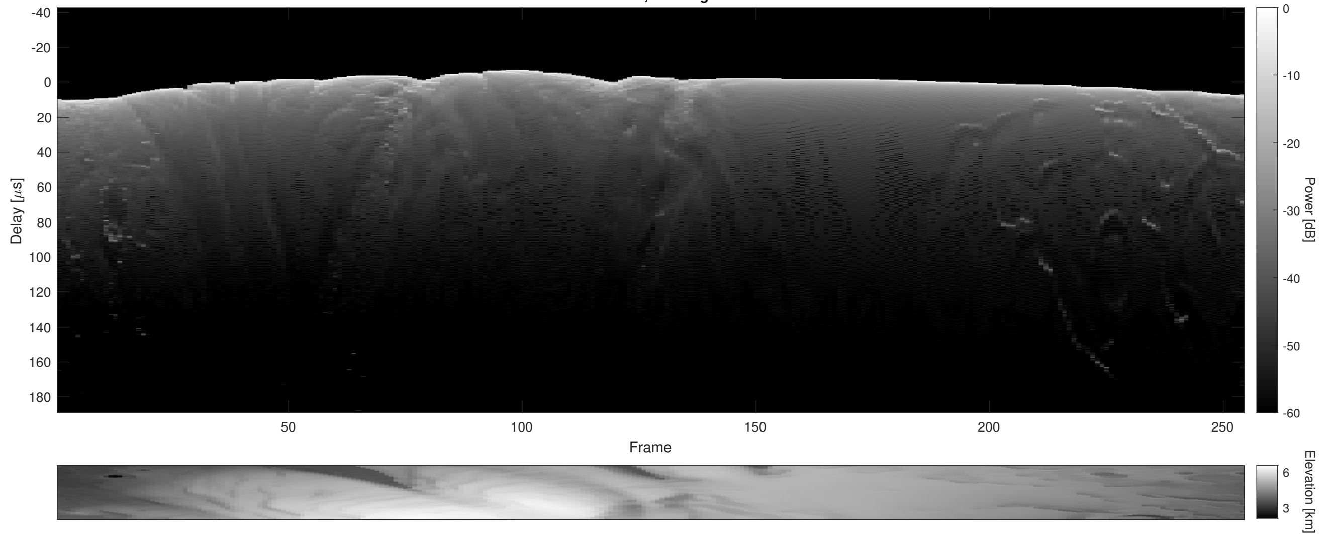
Orbit 10575, Cluttergram
