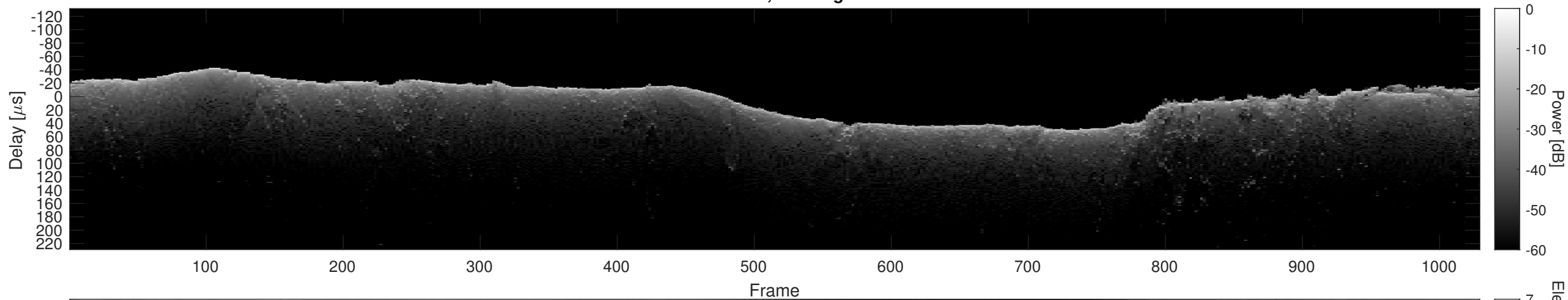
Orbit 10580, Cluttergram
