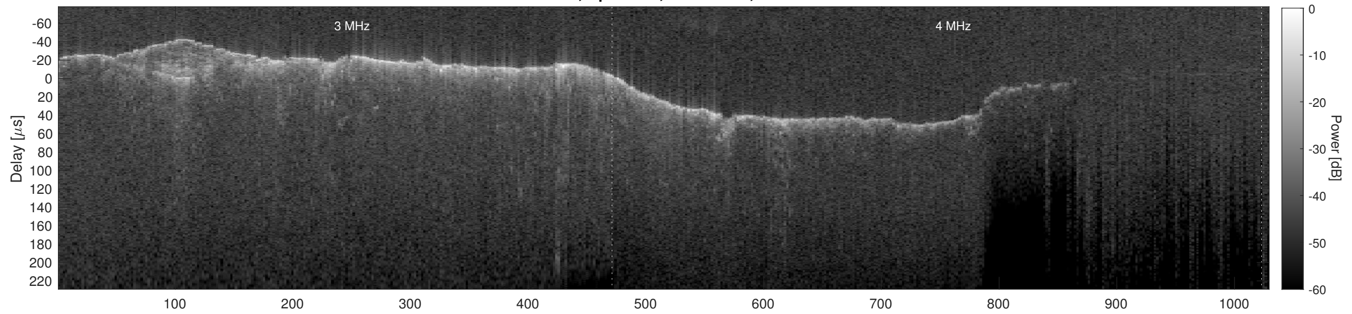
Orbit 10580, Cluttergram
