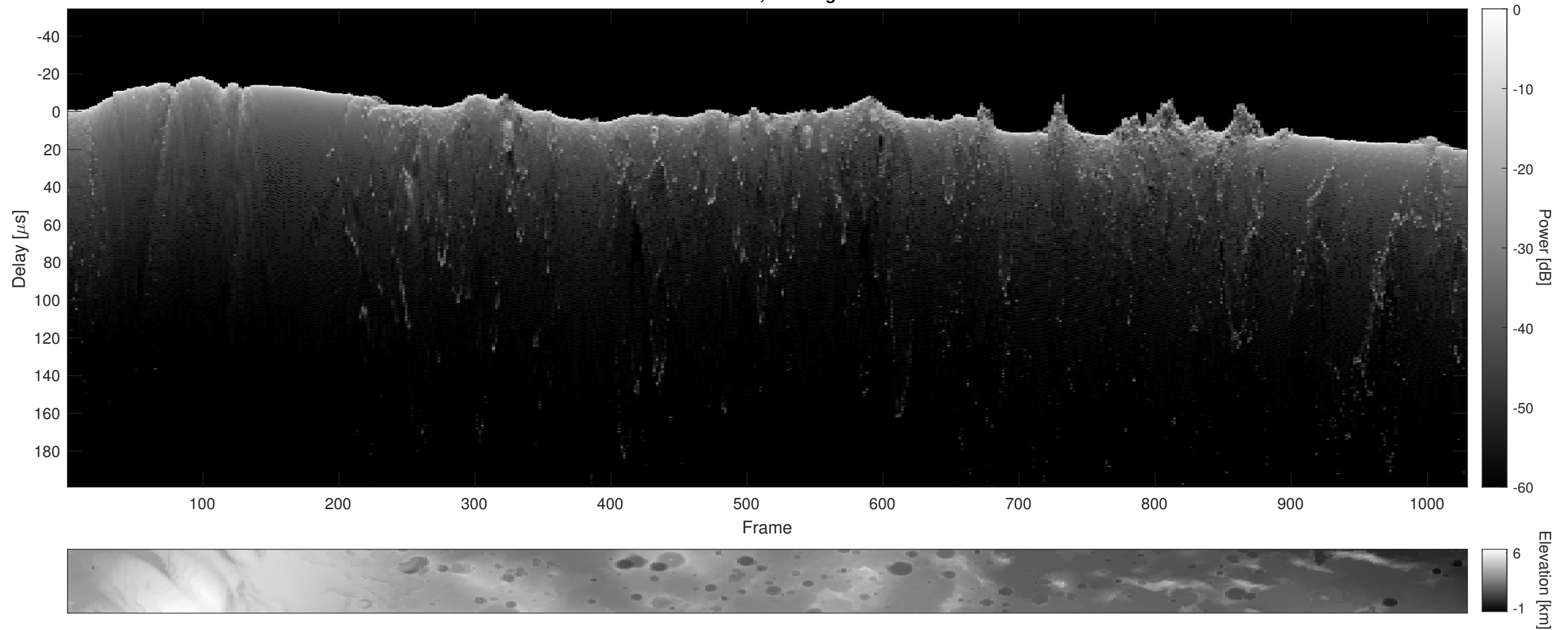
Orbit 10582, Cluttergram
