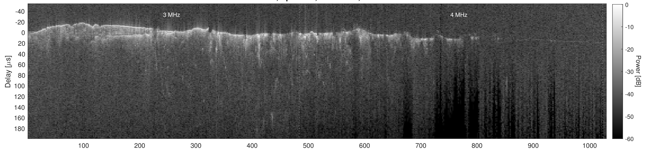
Orbit 10582, Cluttergram
