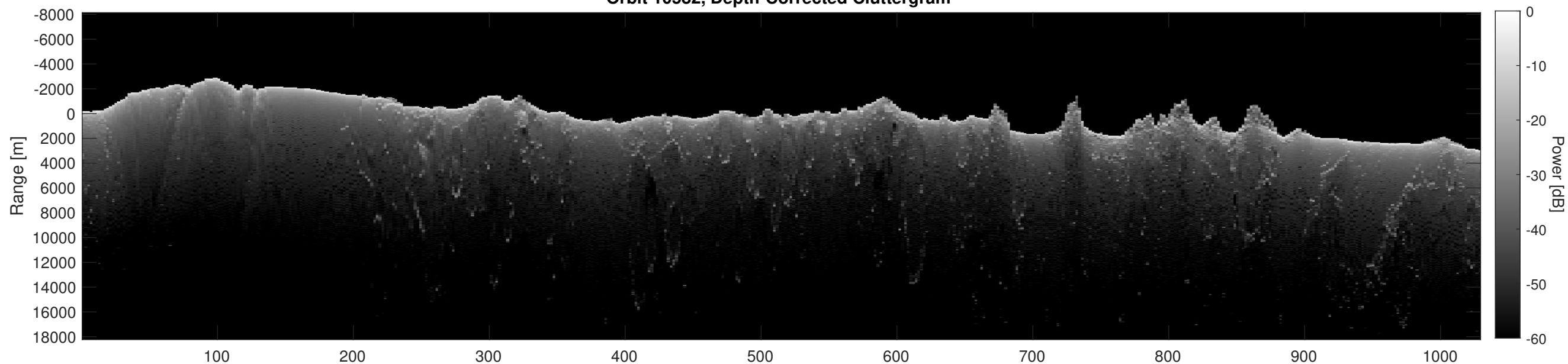
Orbit 10582, Depth-Corrected Cluttergram
