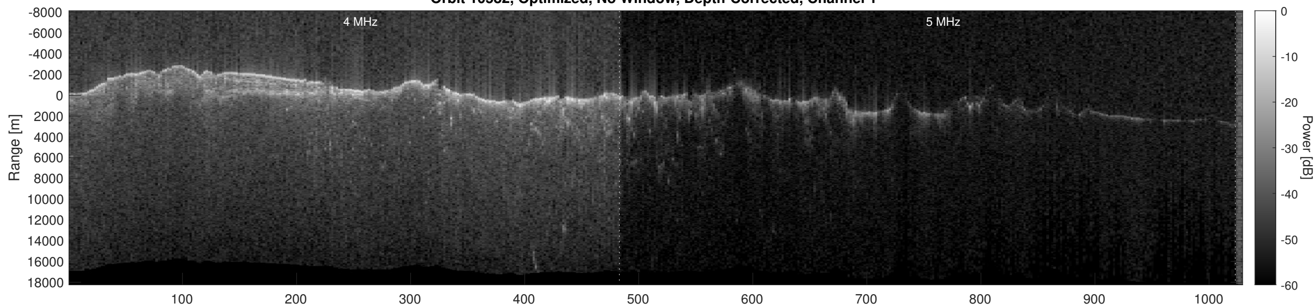
Orbit 10582, Optimized, No Window, Depth-Corrected, Channel 2
