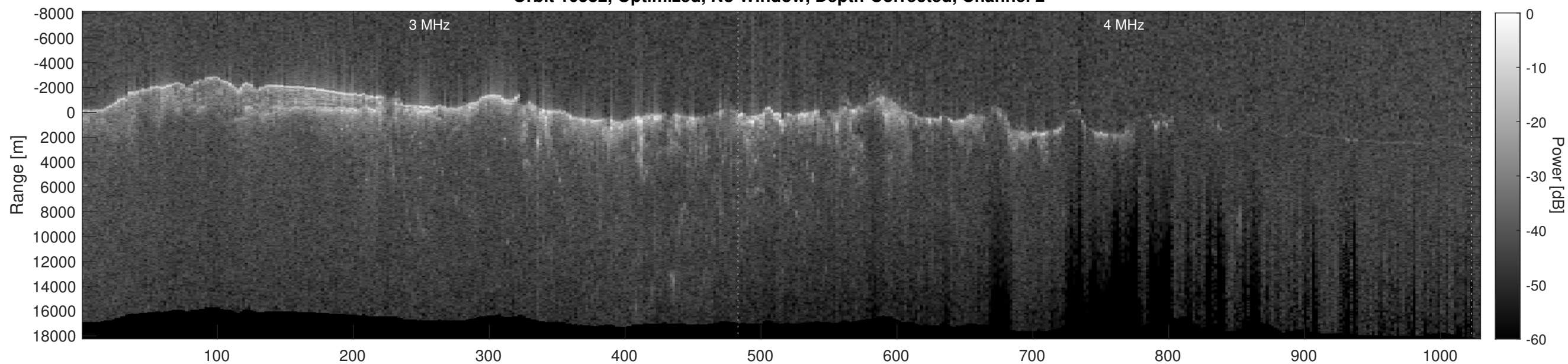
Orbit 10582, Depth-Corrected Cluttergram
