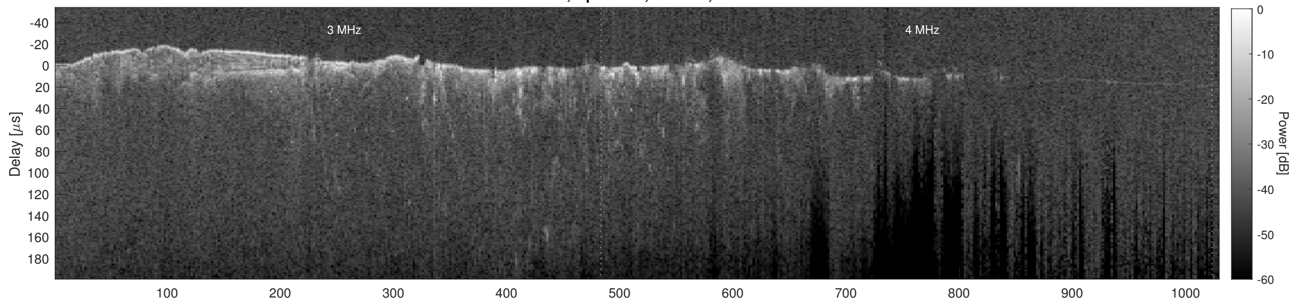
Orbit 10582, Cluttergram
