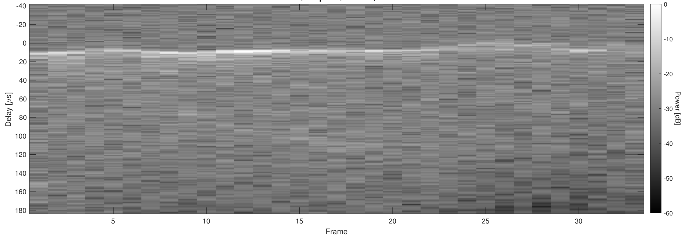
Orbit 10586, Chapman, Window, Channel 2
