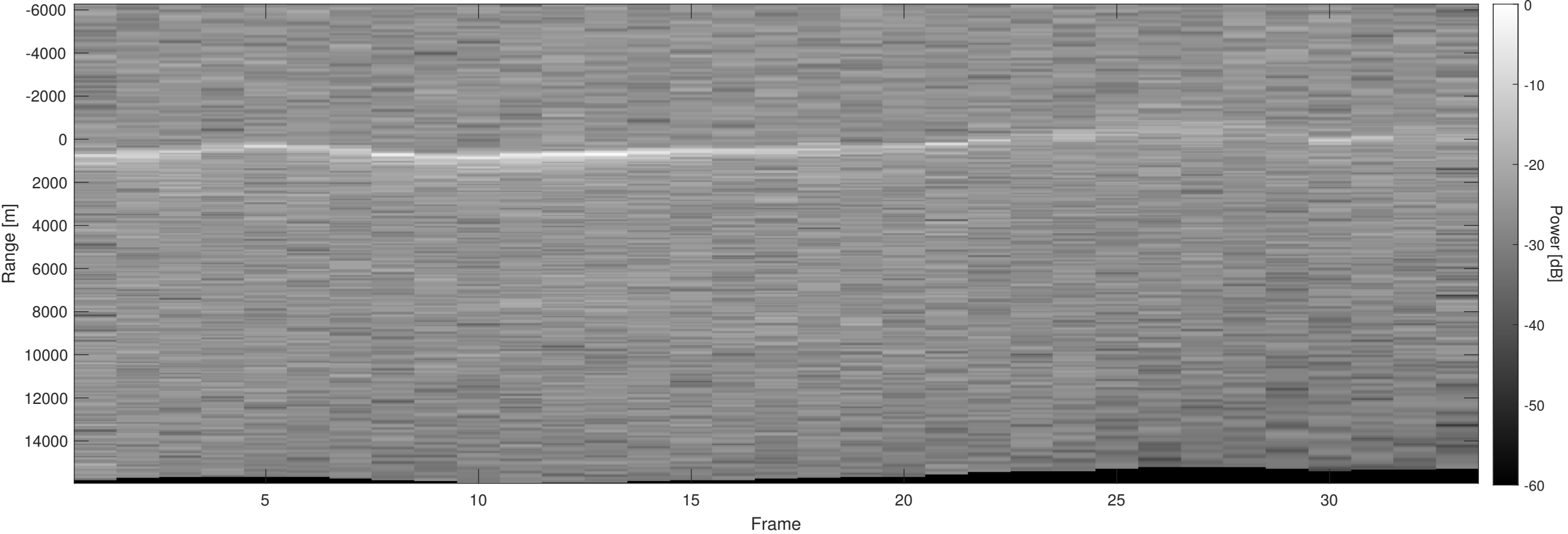
Orbit 10586, Optimized, No Window, Depth-Corrected, Channel 2
