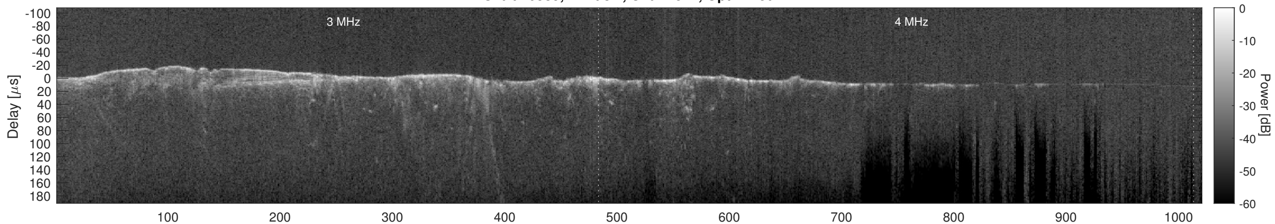
Orbit 10589, Cluttergram
