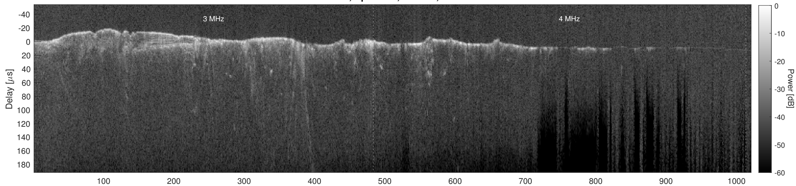
Orbit 10589, Cluttergram
