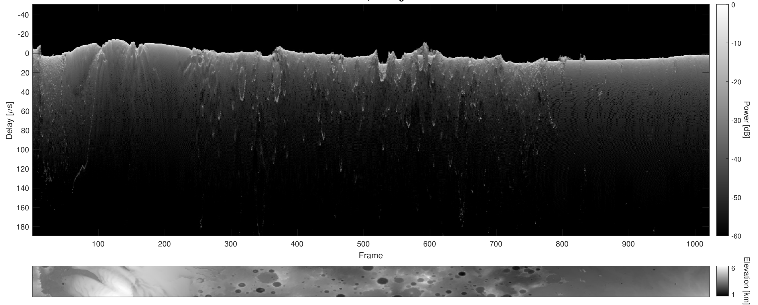
Orbit 10603, Cluttergram
