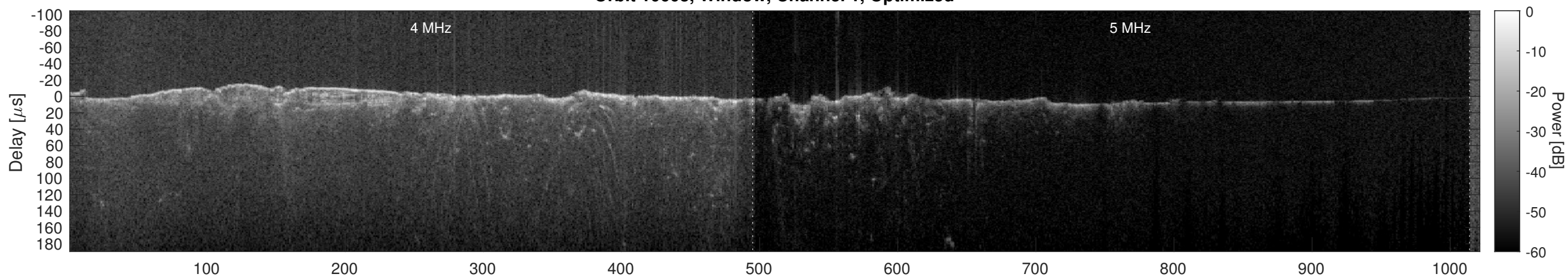
Orbit 10603, Cluttergram
