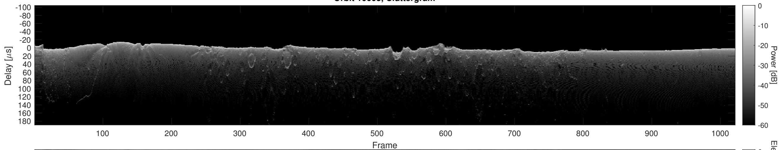
Orbit 10603, Cluttergram
