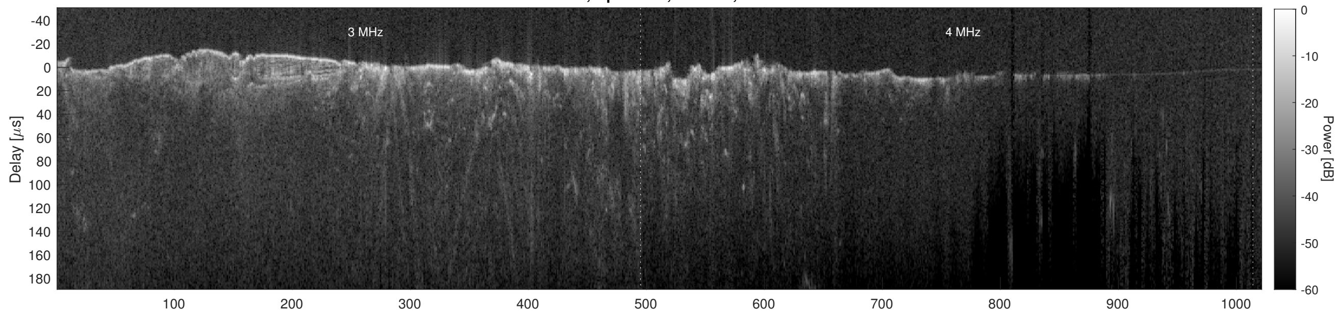
Orbit 10603, Cluttergram
