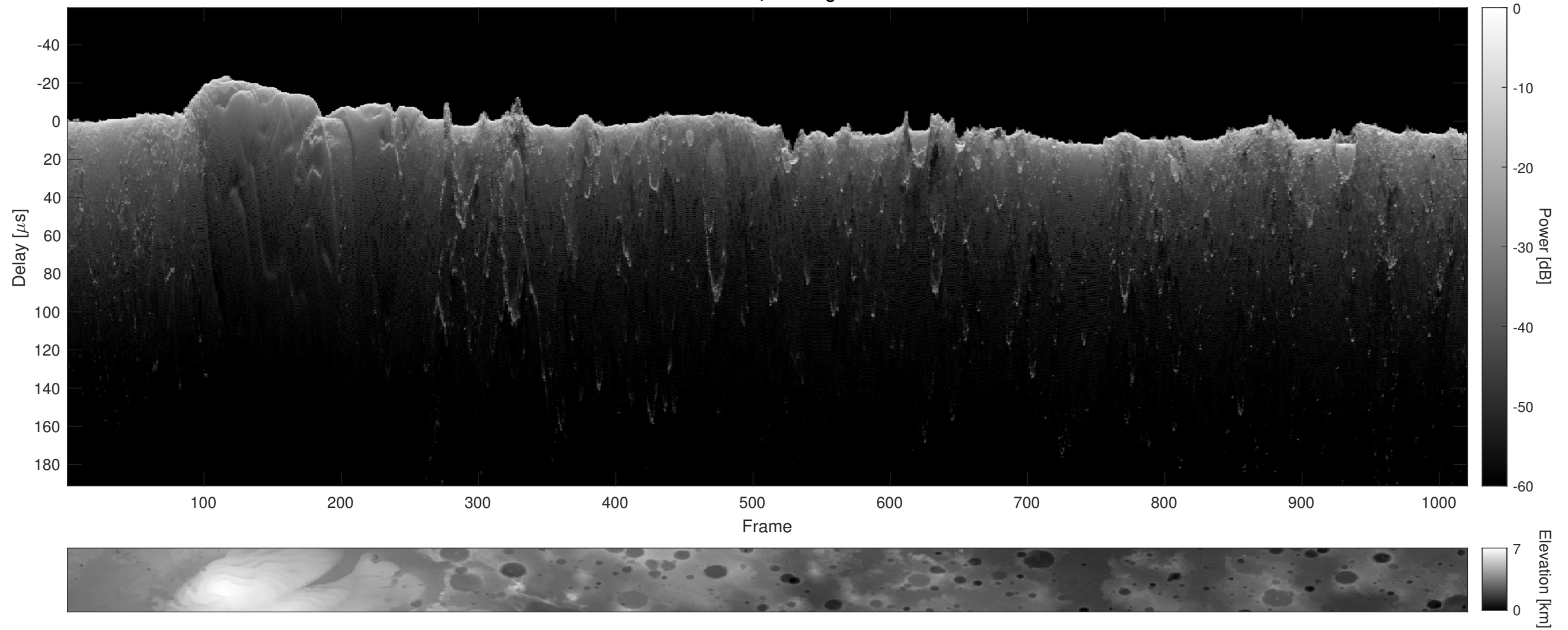
Orbit 10604, Cluttergram
