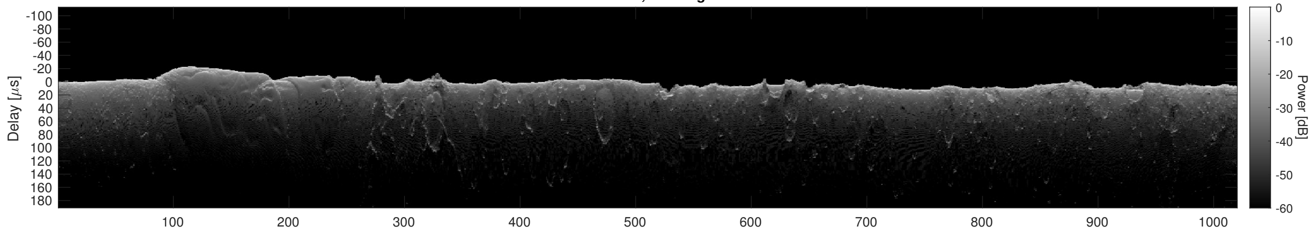
Orbit 10604, Cluttergram
