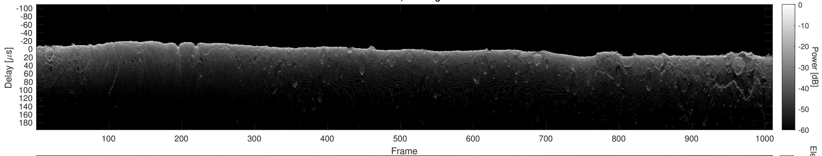
Orbit 10607, Cluttergram
