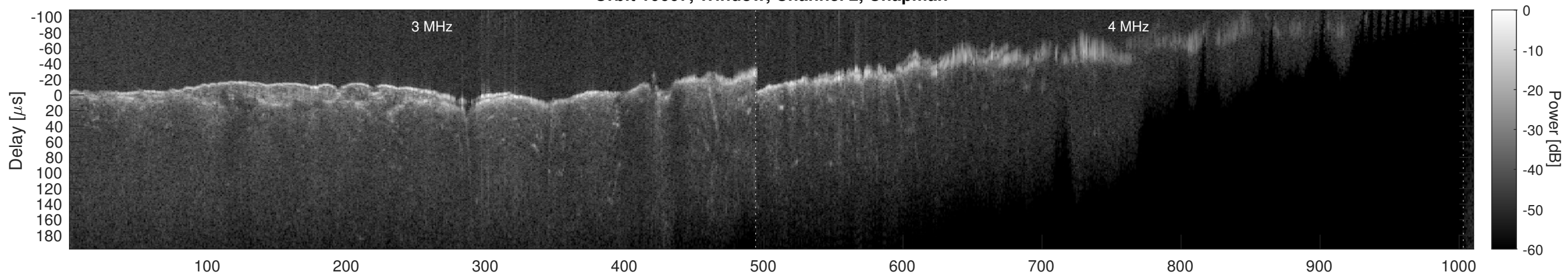
Orbit 10607, Window, Channel 2, Optimized
