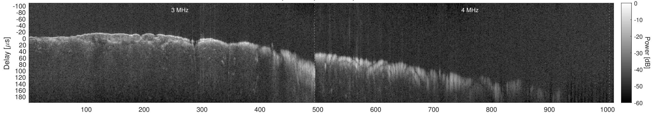
Orbit 10607, Window, Channel 2, Chapman
