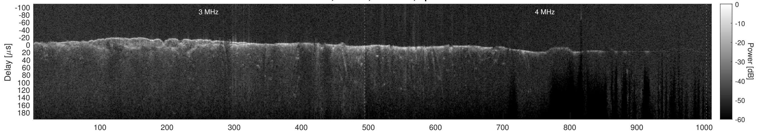
Orbit 10607, Cluttergram
