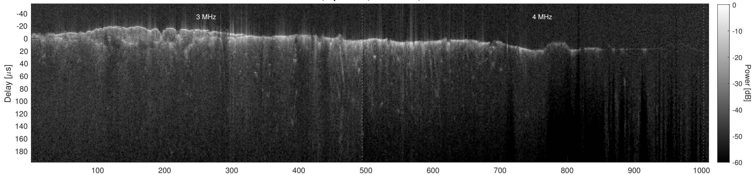
Orbit 10607, Cluttergram
