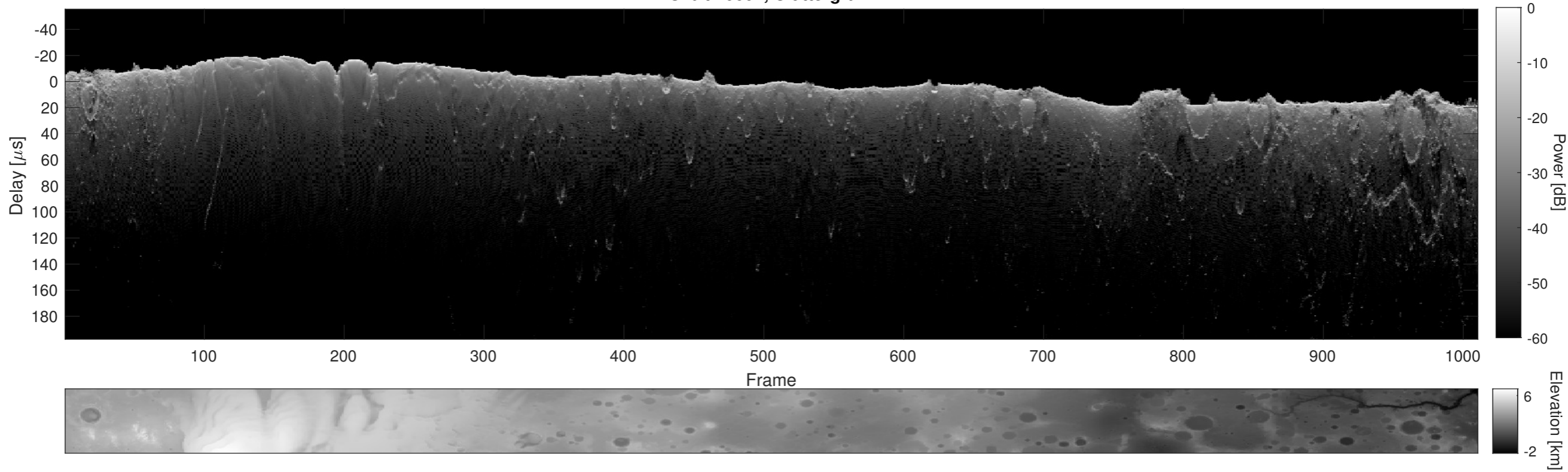
Orbit 10607, Cluttergram
