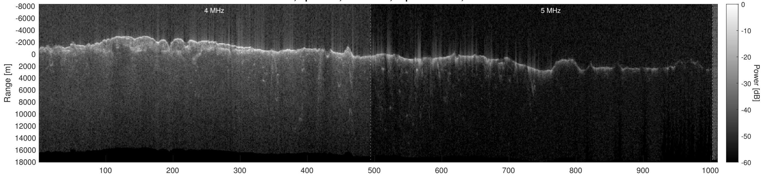
Orbit 10607, Optimized, No Window, Depth-Corrected, Channel 2
