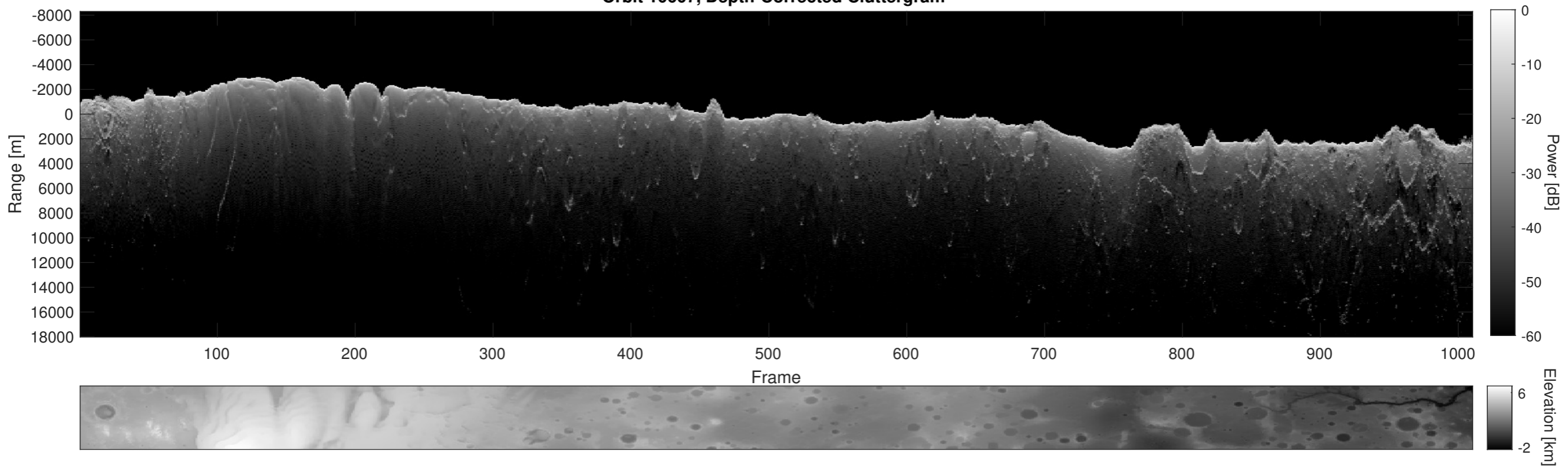
Orbit 10607, Depth-Corrected Cluttergram
