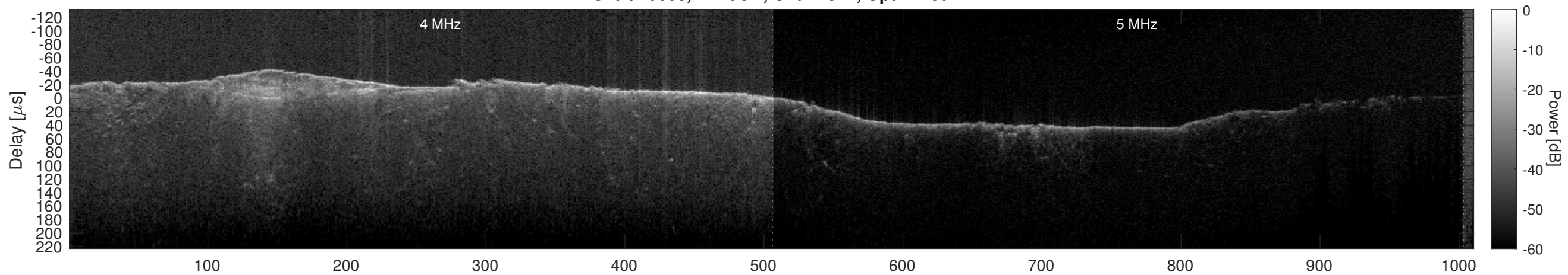
Orbit 10608, Cluttergram
