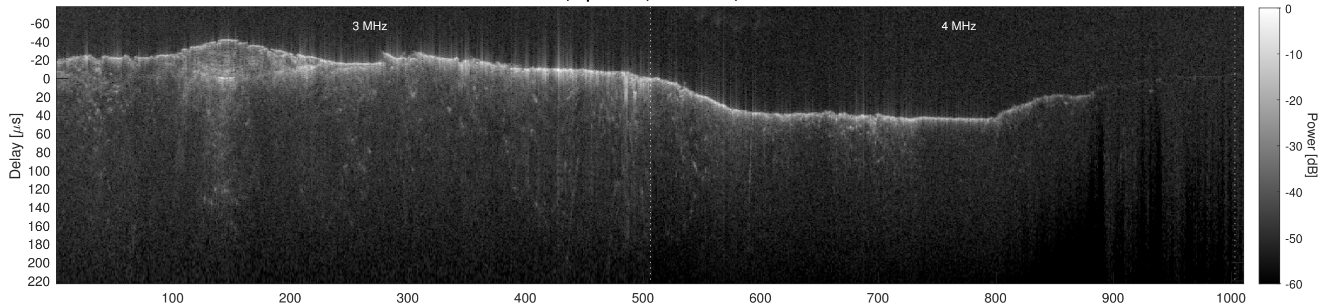
Orbit 10608, Cluttergram
