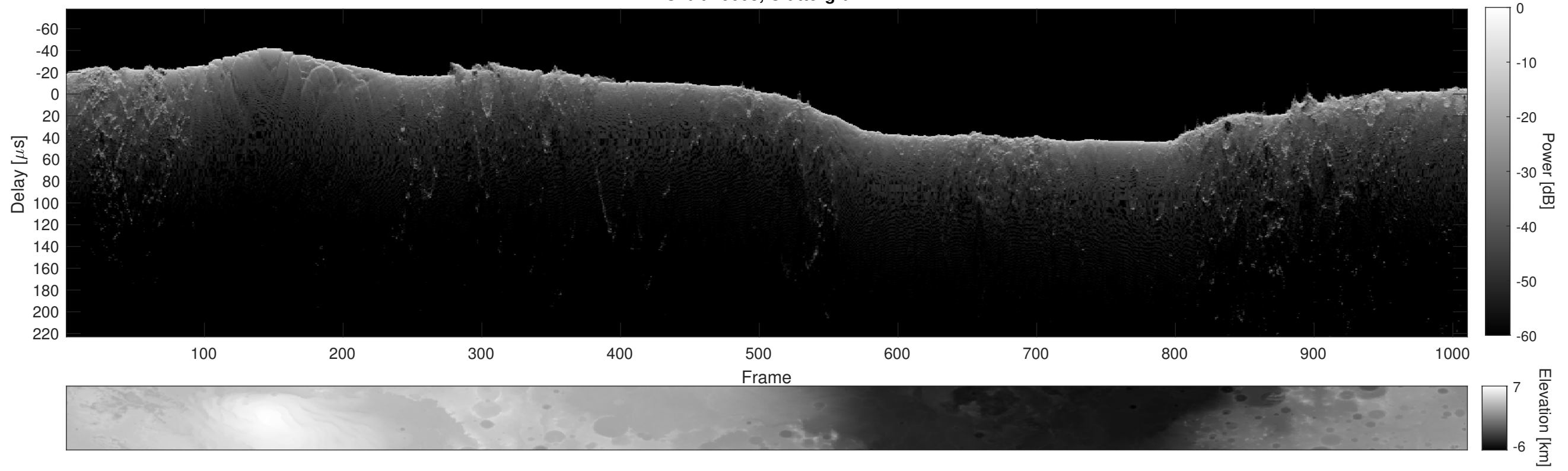
Orbit 10608, Cluttergram
