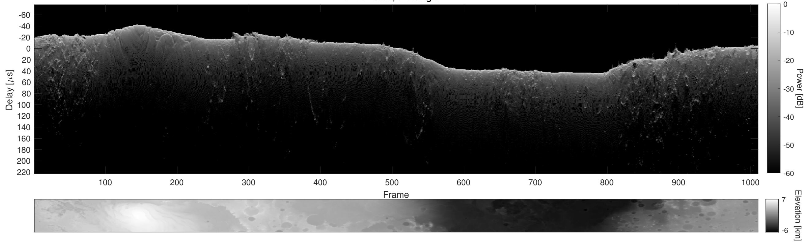
Orbit 10608, Cluttergram
