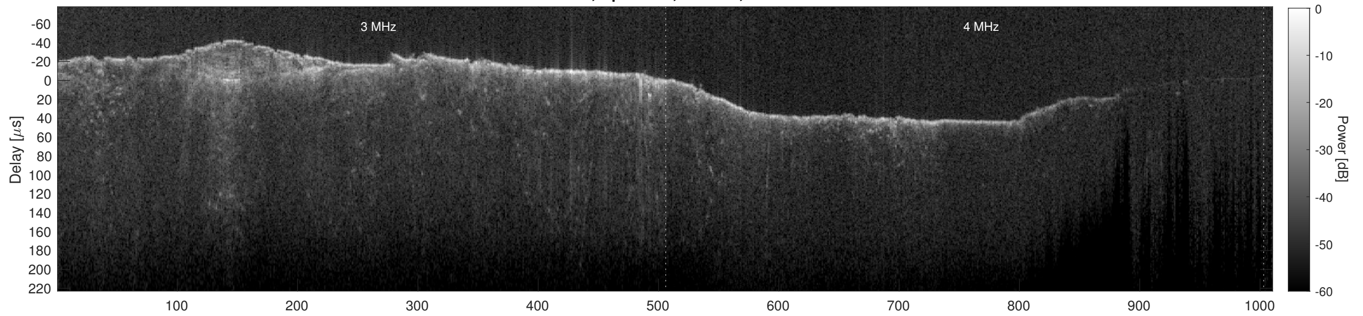
Orbit 10608, Cluttergram
