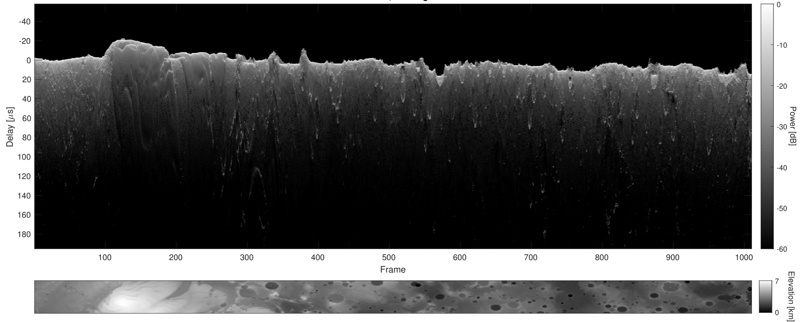
Orbit 10611, Cluttergram
