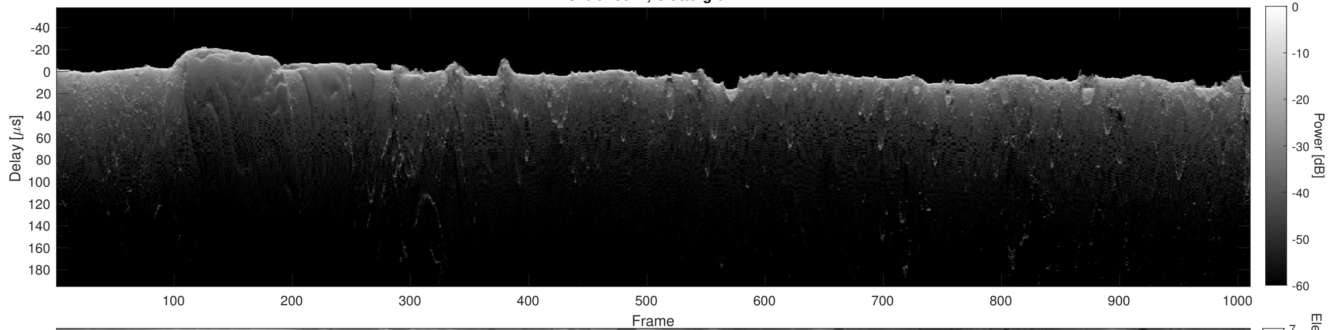
Orbit 10611, Cluttergram
