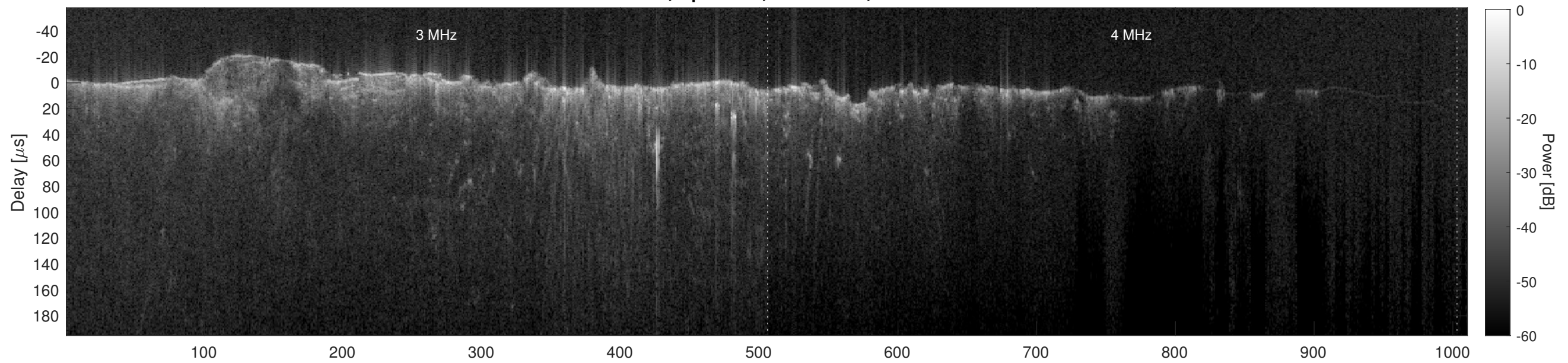
Orbit 10611, Cluttergram
