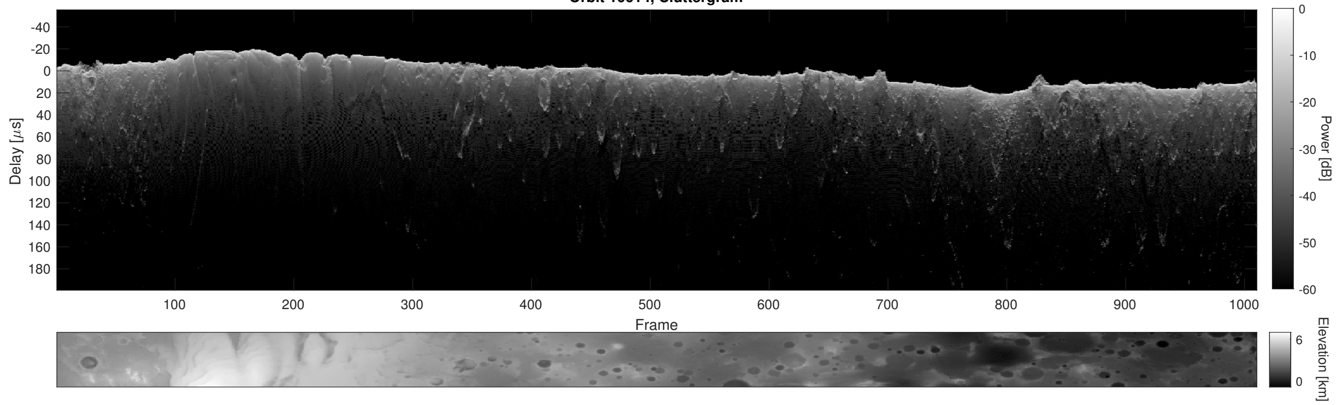
Orbit 10614, Cluttergram
