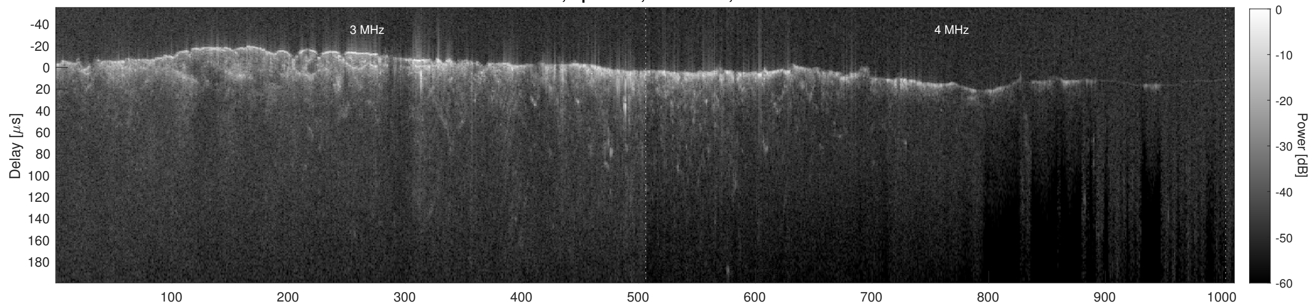
Orbit 10614, Cluttergram
