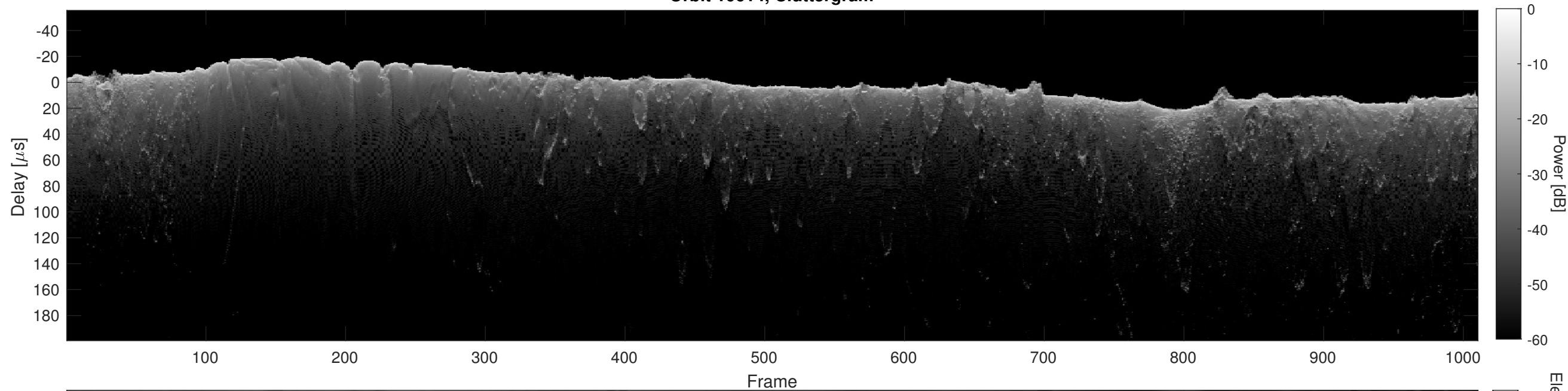
Orbit 10614, Cluttergram
