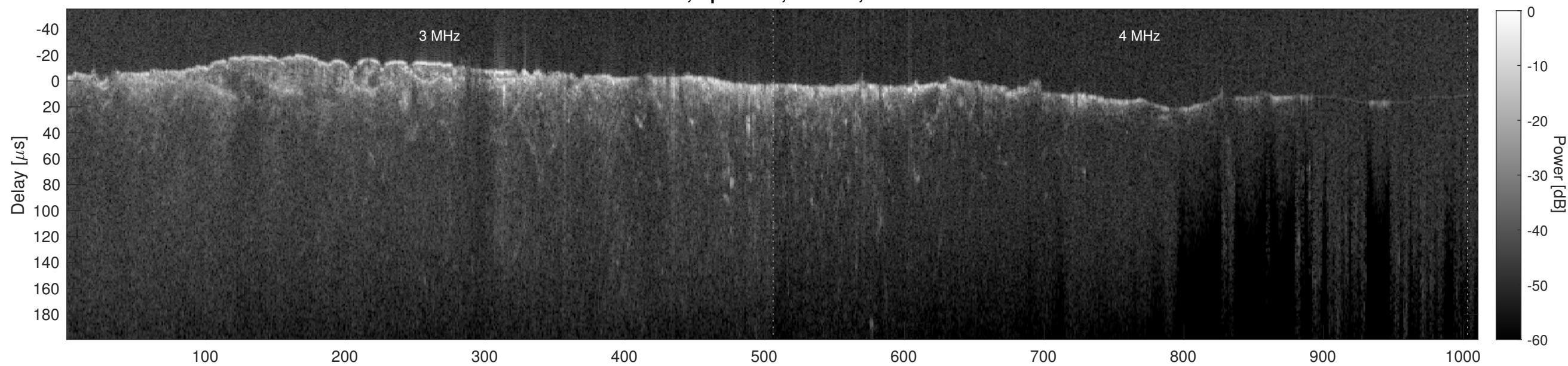
Orbit 10614, Cluttergram
