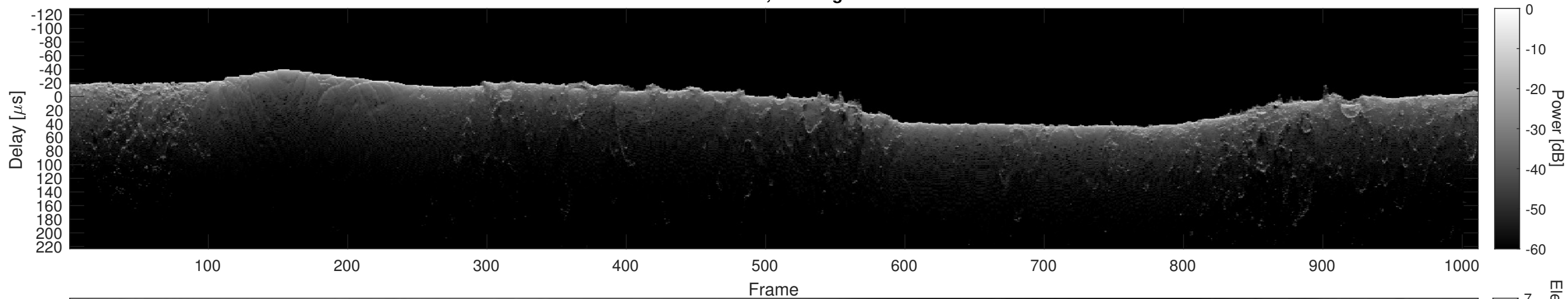
Orbit 10615, Cluttergram
