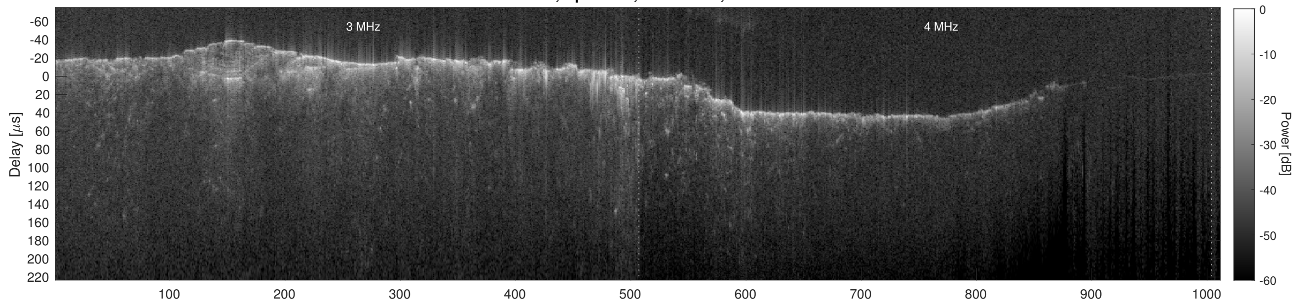
Orbit 10615, Cluttergram
