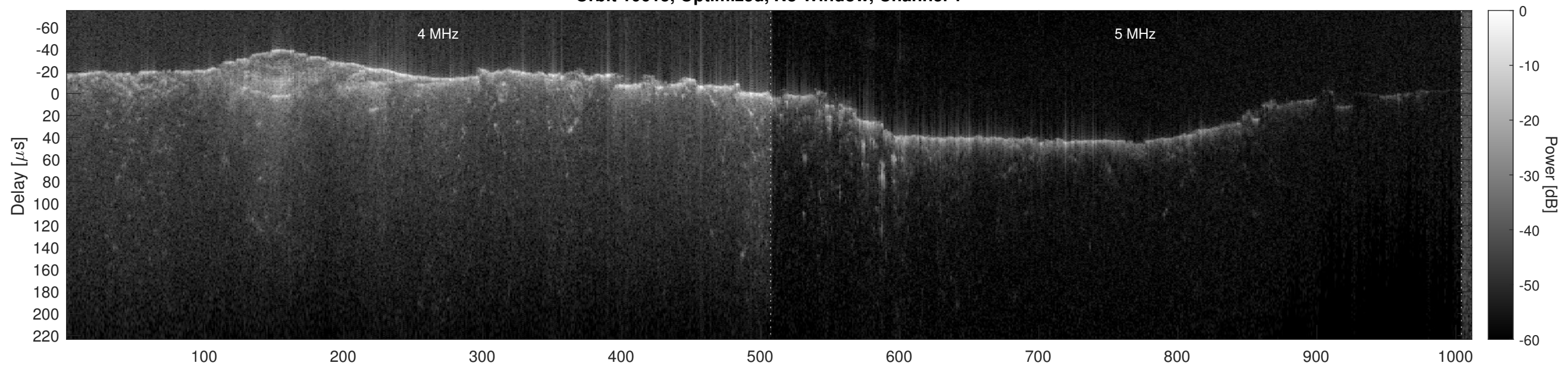
Orbit 10615, Optimized, No Window, Channel 2
