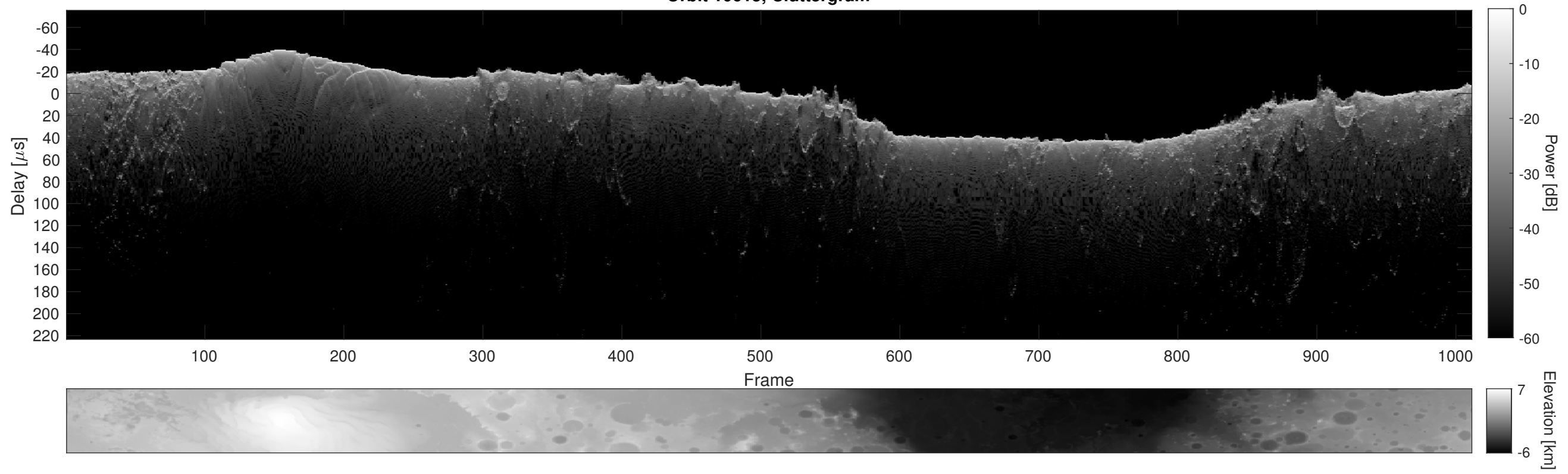
Orbit 10615, Cluttergram
