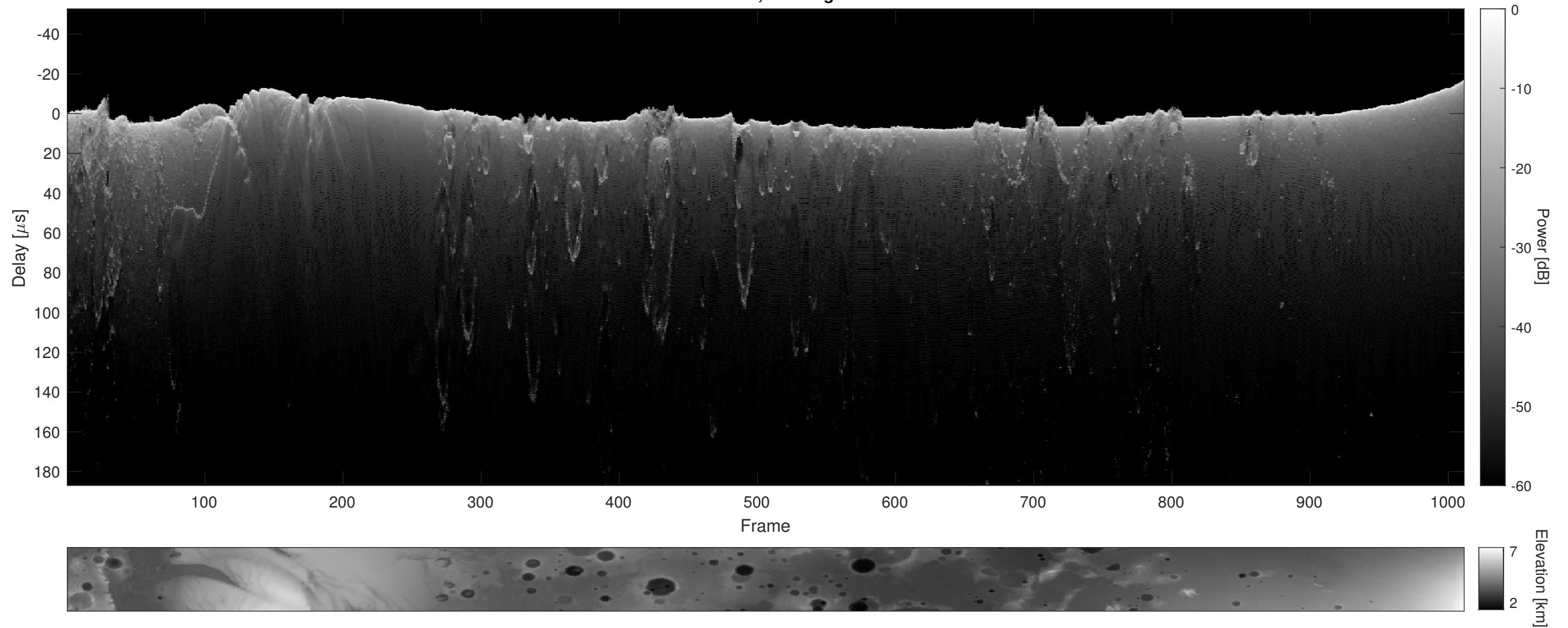
Orbit 10617, Cluttergram
