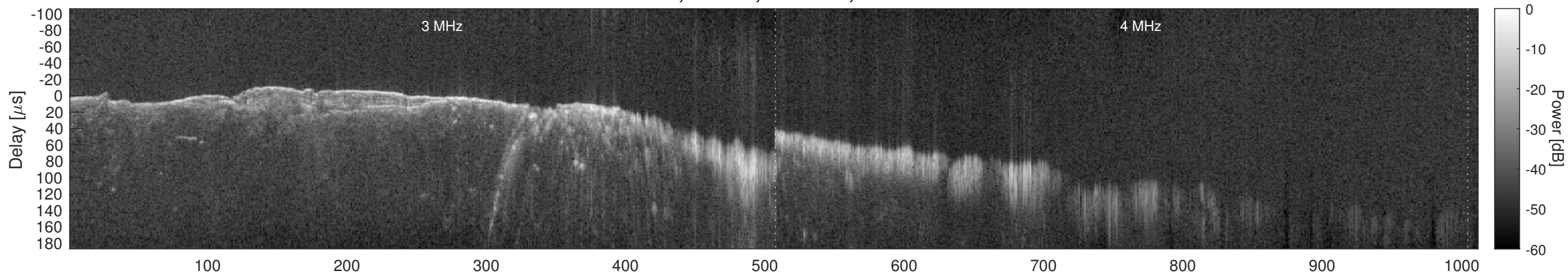
Orbit 10617, Window, Channel 2, Chapman
