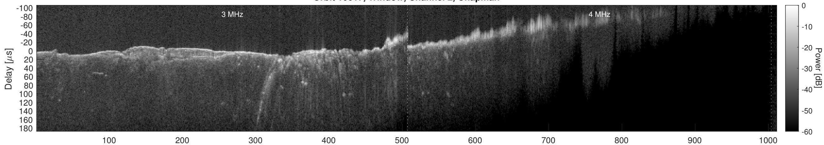
Orbit 10617, Window, Channel 2, Optimized
