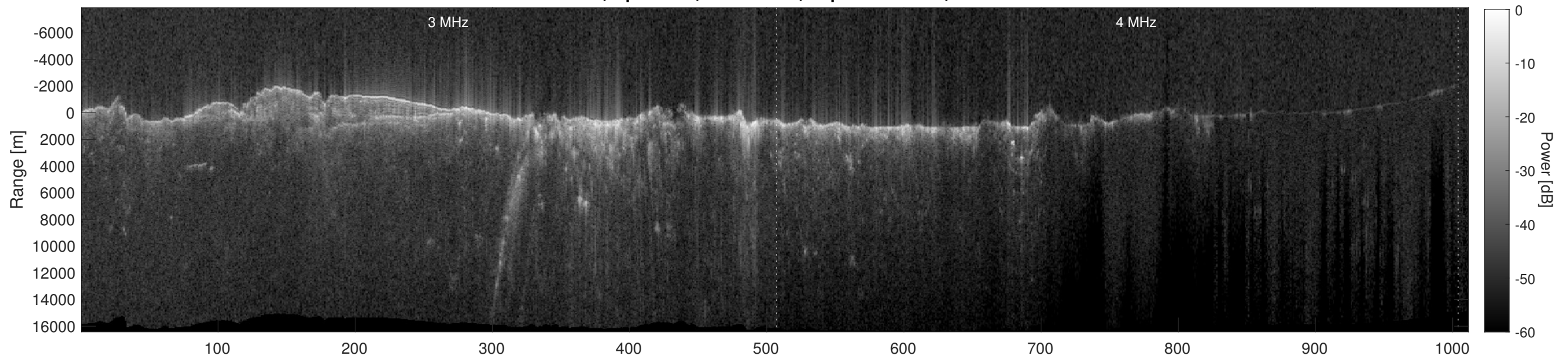
Orbit 10617, Depth-Corrected Cluttergram
