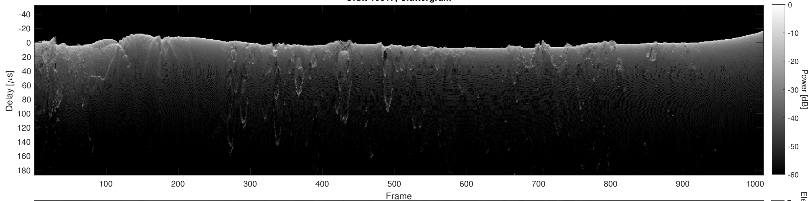
Orbit 10617, Cluttergram
