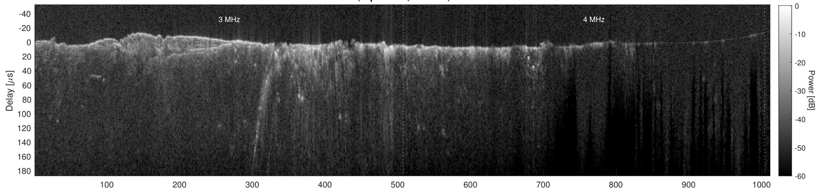
Orbit 10617, Cluttergram
