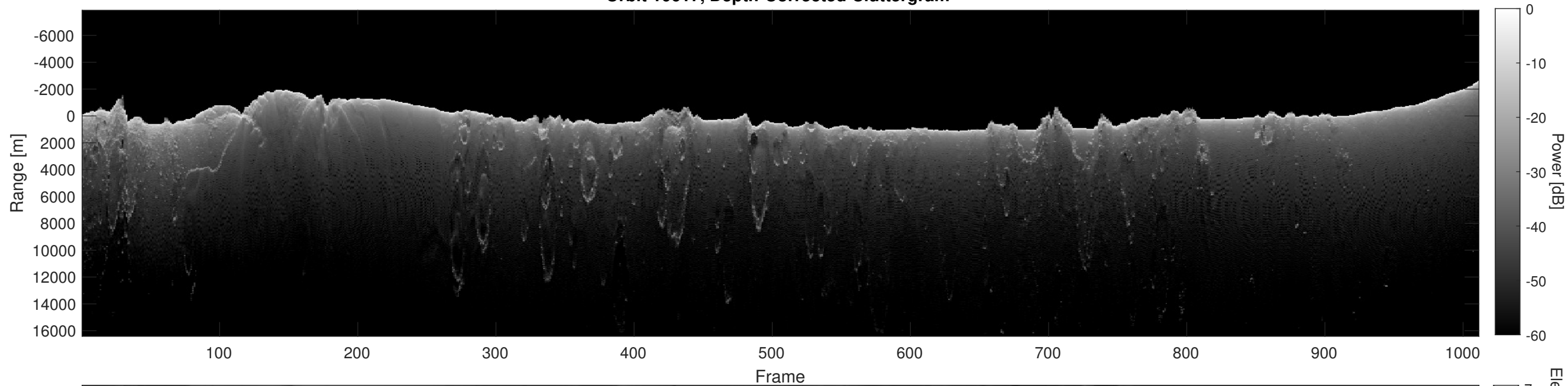
Orbit 10617, Depth-Corrected Cluttergram
