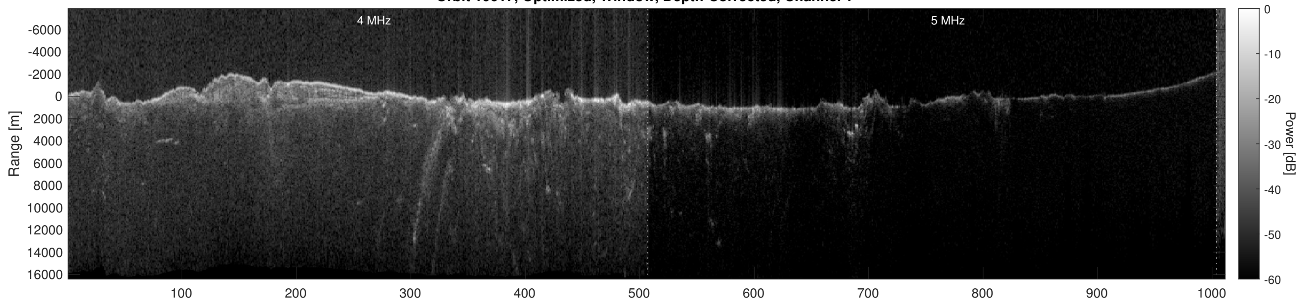
Orbit 10617, Optimized, Window, Depth-Corrected, Channel 2
