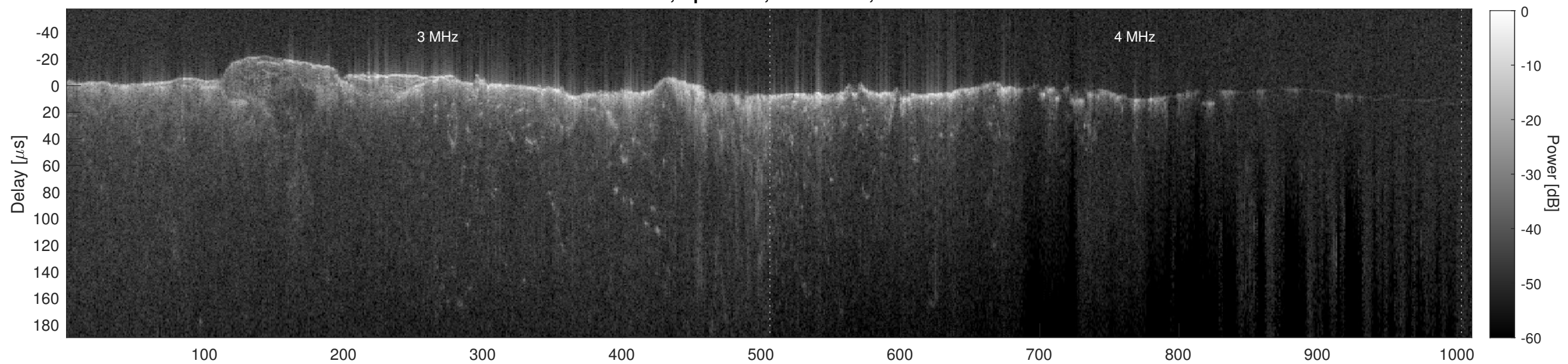
Orbit 10618, Cluttergram
