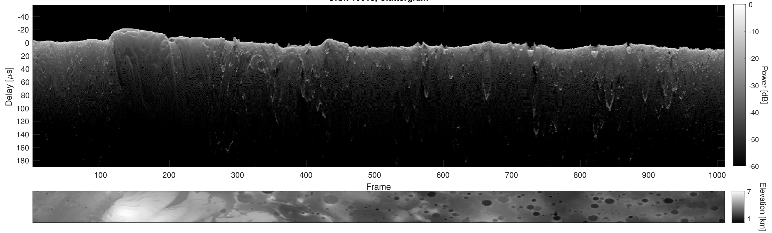
Orbit 10618, Cluttergram
