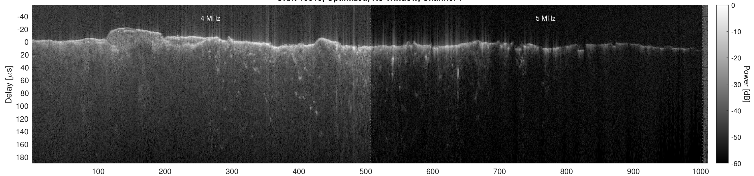
Orbit 10618, Optimized, No Window, Channel 2
