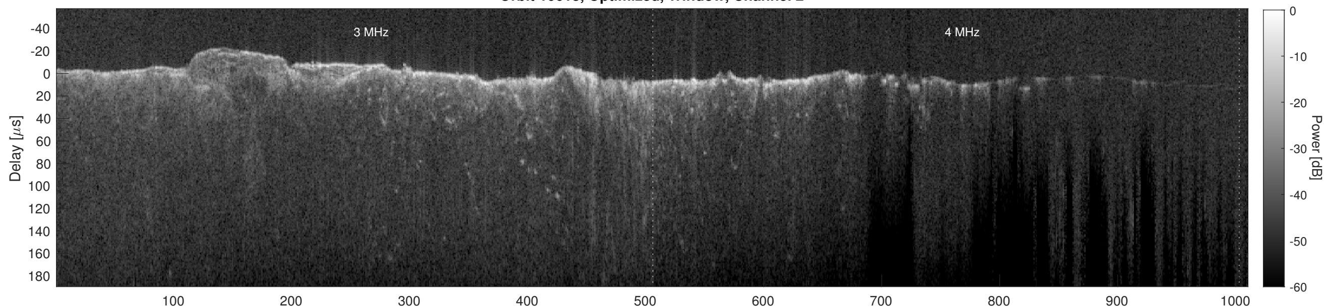
Orbit 10618, Cluttergram
