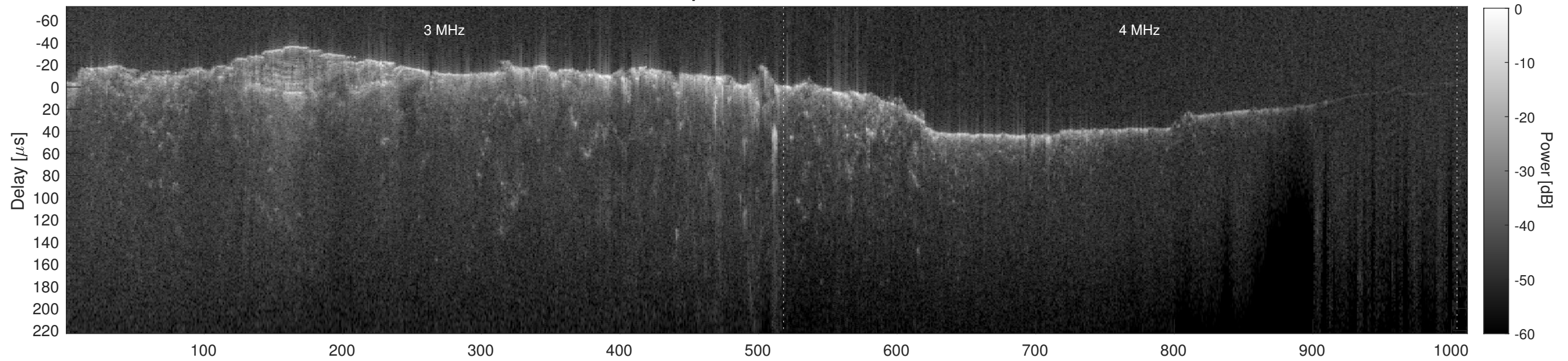
Orbit 10622, Cluttergram
