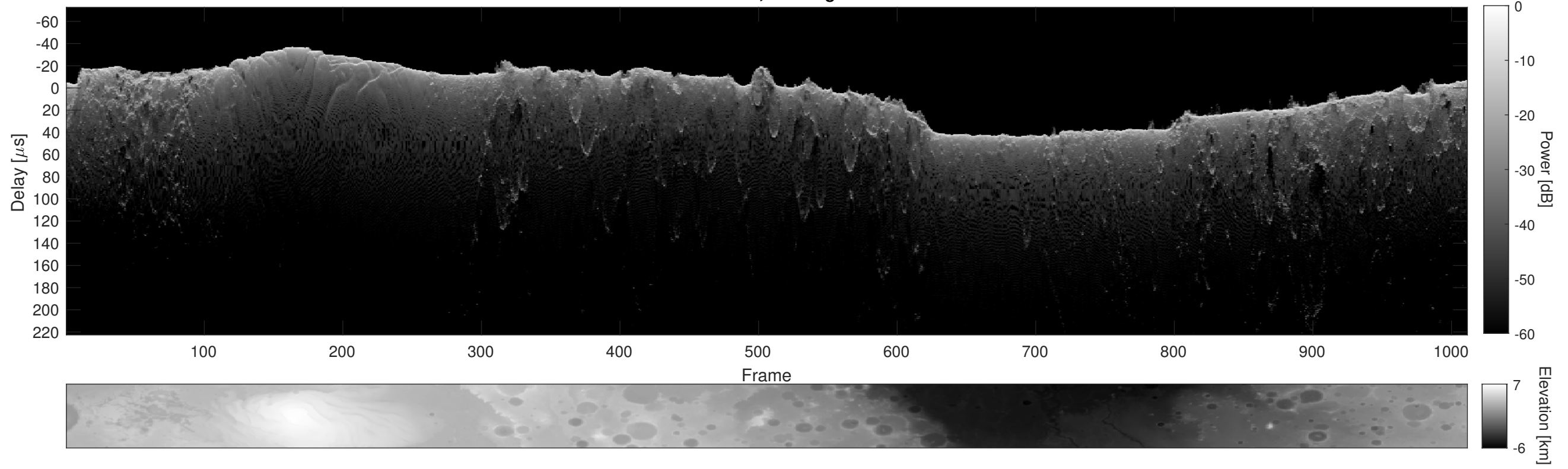
Orbit 10622, Cluttergram
