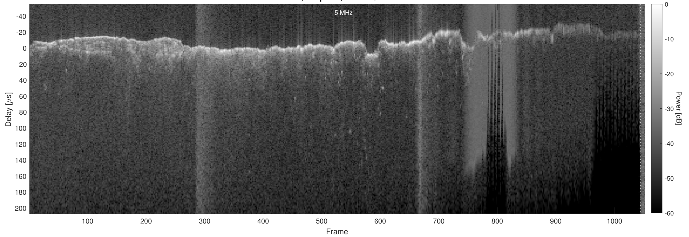
Orbit 10623, Chapman, Window, Channel 2
