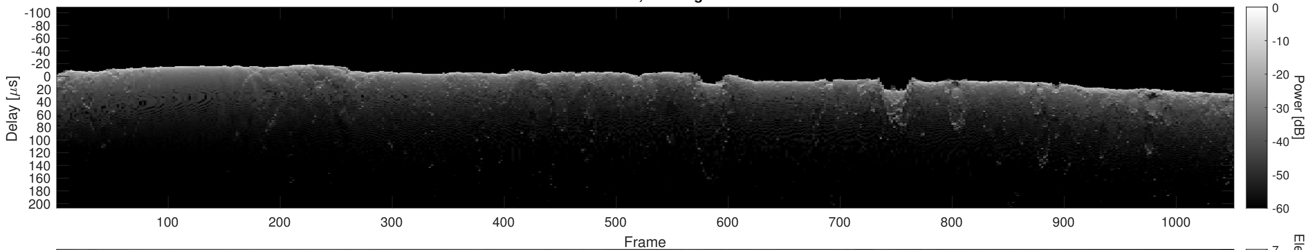
Orbit 10623, Cluttergram
