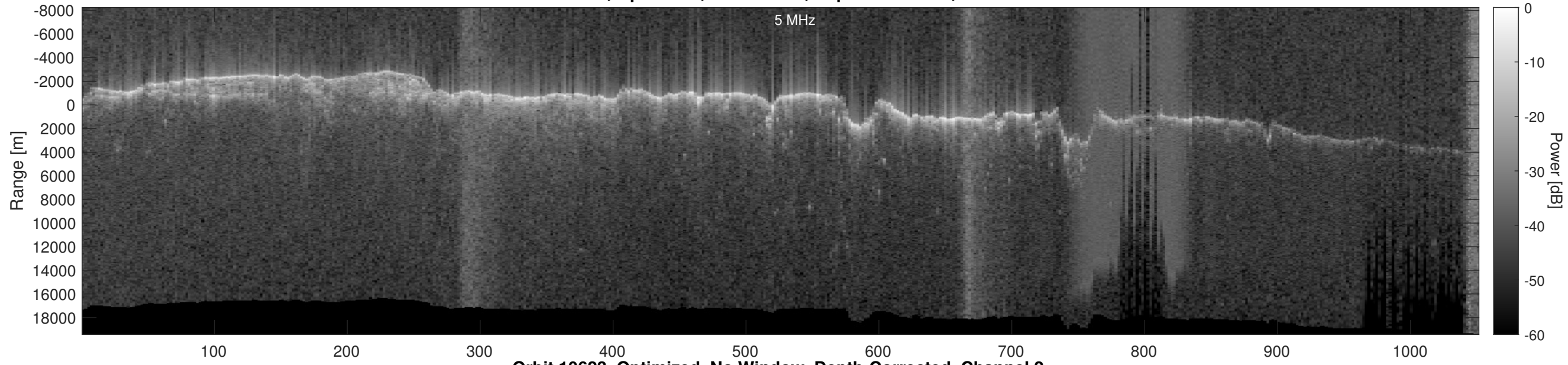
Orbit 10623, Optimized, No Window, Depth-Corrected, Channel 2
