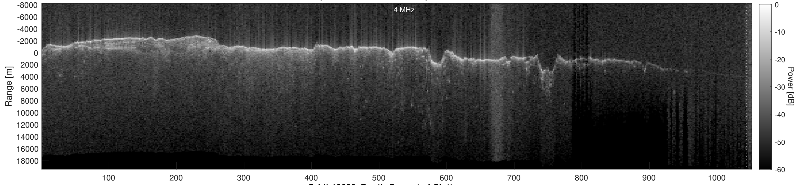
Orbit 10623, Depth-Corrected Cluttergram
