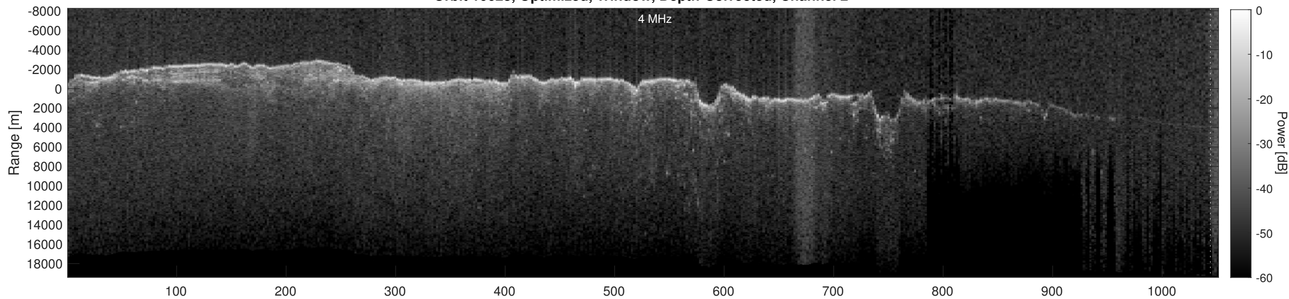
Orbit 10623, Depth-Corrected Cluttergram
