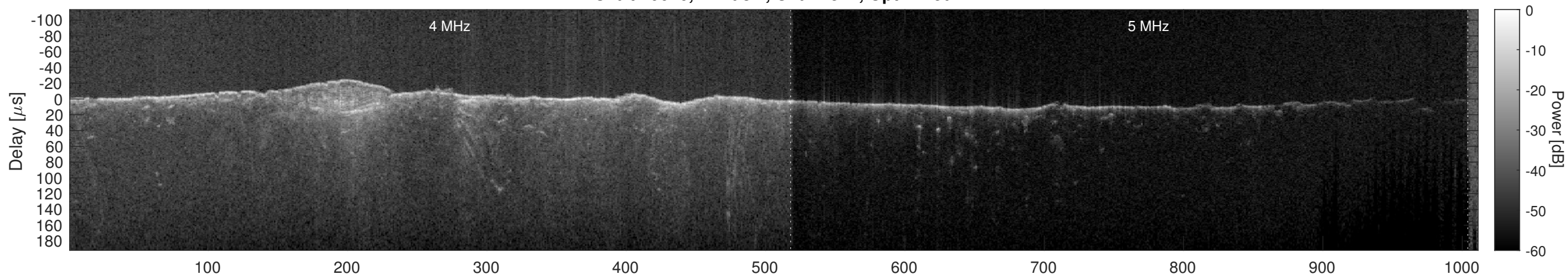
Orbit 10626, Cluttergram
