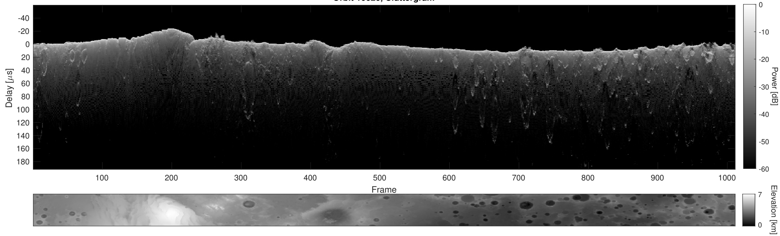
Orbit 10626, Cluttergram
