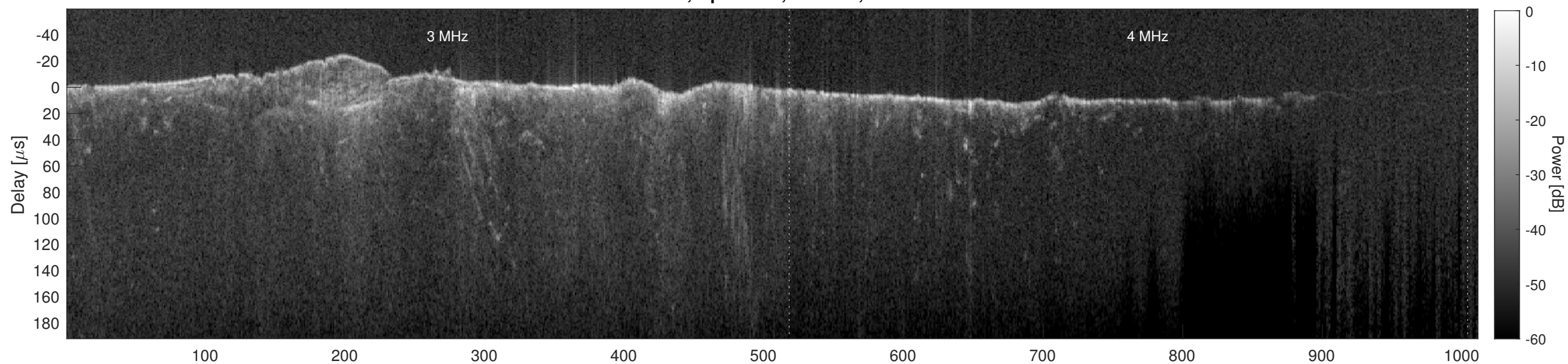
Orbit 10626, Cluttergram
